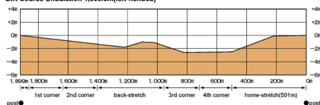
Dirt Course Undulation 1,899.0m(left-handed)
